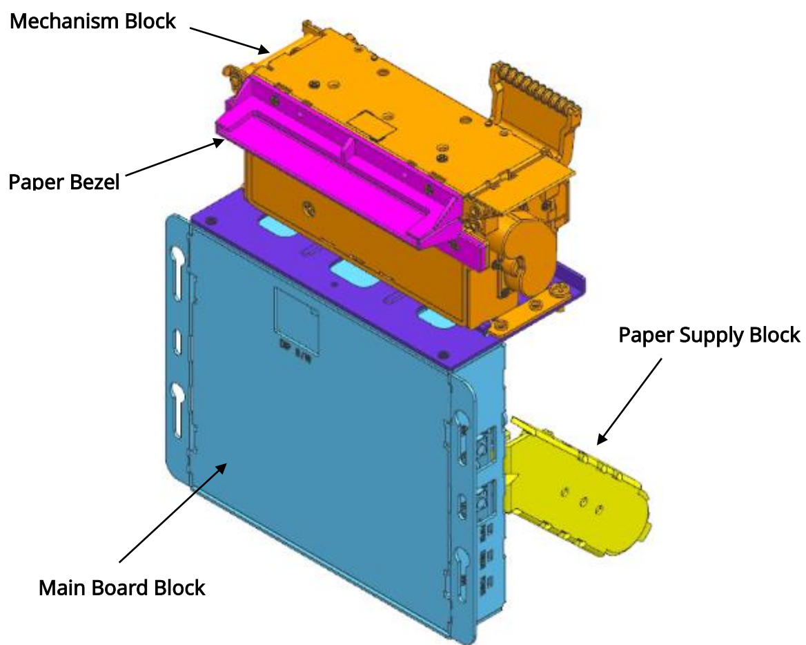
Vertical Type
